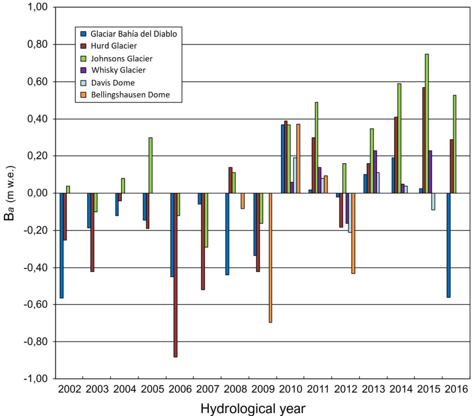
Fig. 11. Comparison of the climatic annual mass balances of various glaciers in the periphery of the northern Antarctic Peninsula. Bahía del Diablo, Hurd and Johnsons glaciers are the only ones that currently have more than 20 years of continuous mass balance records in the WGMS database for Region 19-Antarctic and Subantarctic. Glaciar Bahía del Diablo is located on Vega Island, and Davies Dome and Whisky Glacier on James Ross Island, both to the NE of the AP. Bellingshausen Dome is located on King George Island, SSI, some 100 km away from our study glaciers, Hurd and Johnsons.
